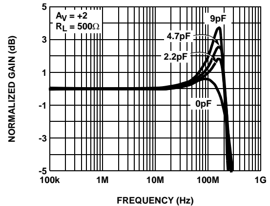
FIGURE 2. GAIN vs FREQUENCY FOR VARIOUS C_{\text{LOAD}}
