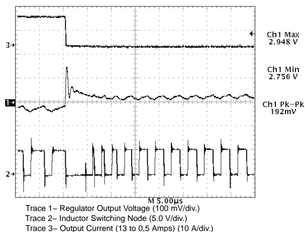
Figure 11. CS5157H Demonstration Board Response to 13 A Load Turn Off (Output Set for 2.8 V). V^2 Control Topology Immediately Connects Inductor to Ground, Providing 0% Duty Cycle. Regulation is Achieved in Less Than 10 \mu s
