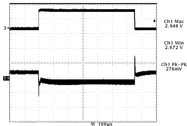
Figure 9. CS5157H Demonstration Board Response to a 0.5 to 13 A Load Pulse (Output Set for 2.8 V)
