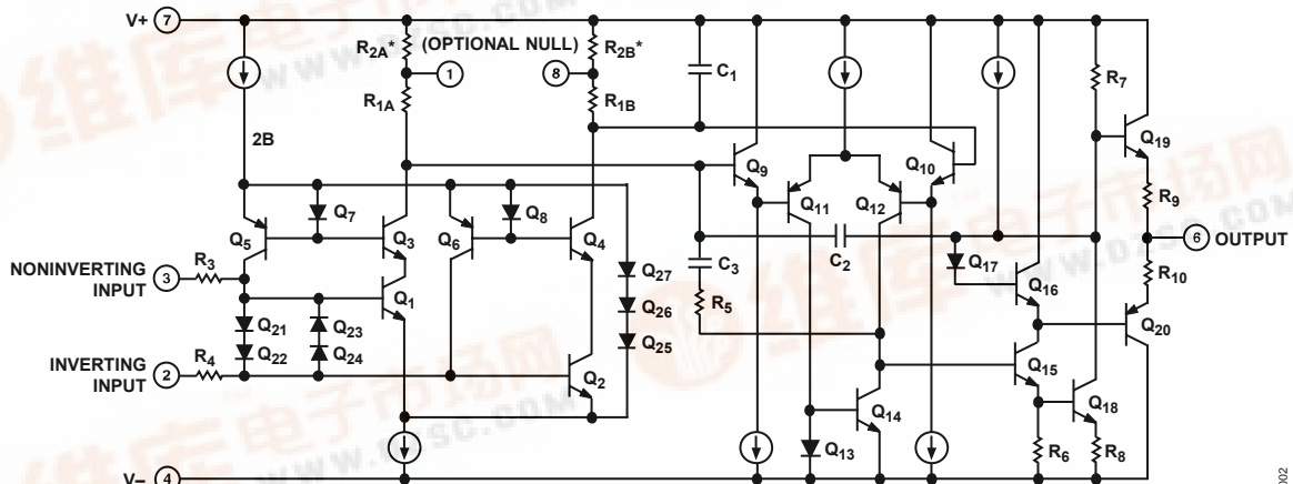
Figure 2. Simplified Schematic
