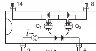
C47 is the same configuration except Q 2 has been replaced with a wire short
