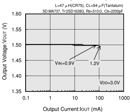
XC6368A151MR (100kHz, 1.5V)
