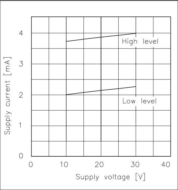
Figure 6. Supply current vs. supply voltage
