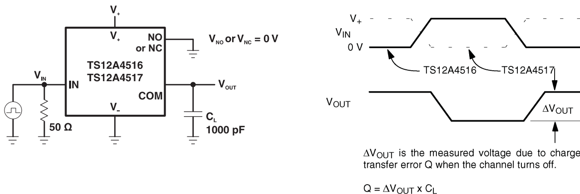
Figure 1. Charge Injection
