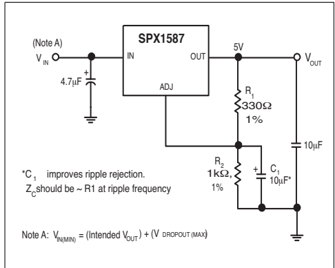
Figure 8. Improving Ripple Rejection
