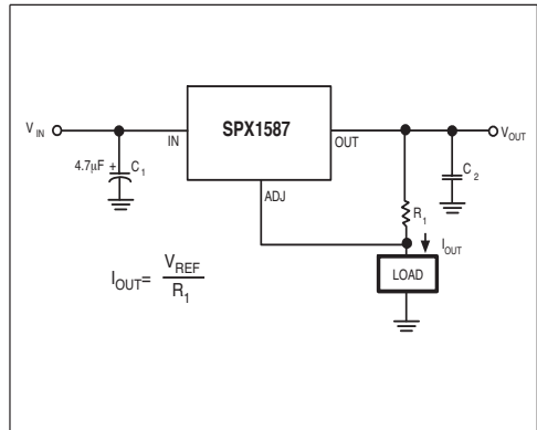
Figure 6. Current Source
