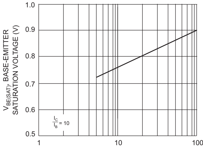
I_C , COLLECTOR CURRENT (mA) Fig. 9, Typical Base-Emitter Saturation Voltage vs. Collector Current (PNP-3906)
