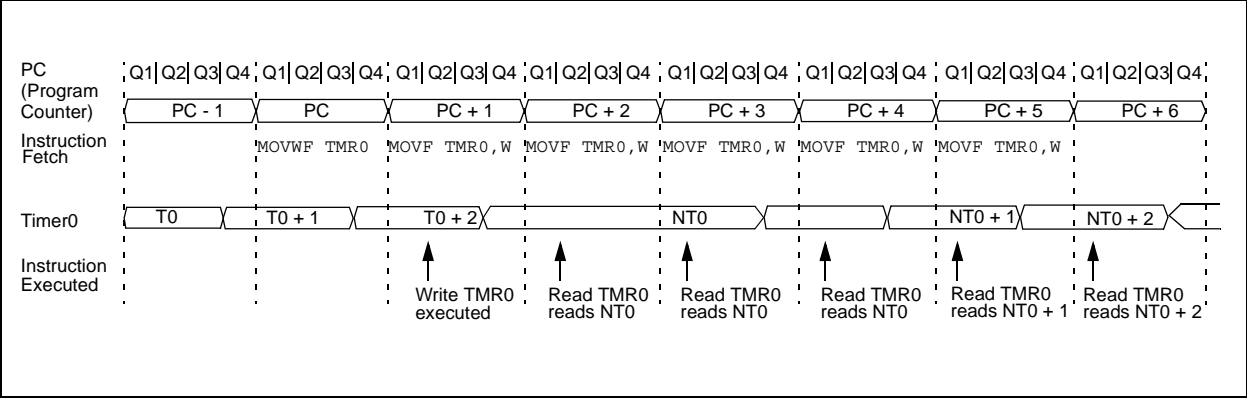
FIGURE 6-3: TIMER0 TIMING: INTERNAL CLOCK/PRESCALE 1:2
