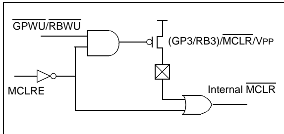
FIGURE 10-7: \overline{\text{MCLR}} SELECT
