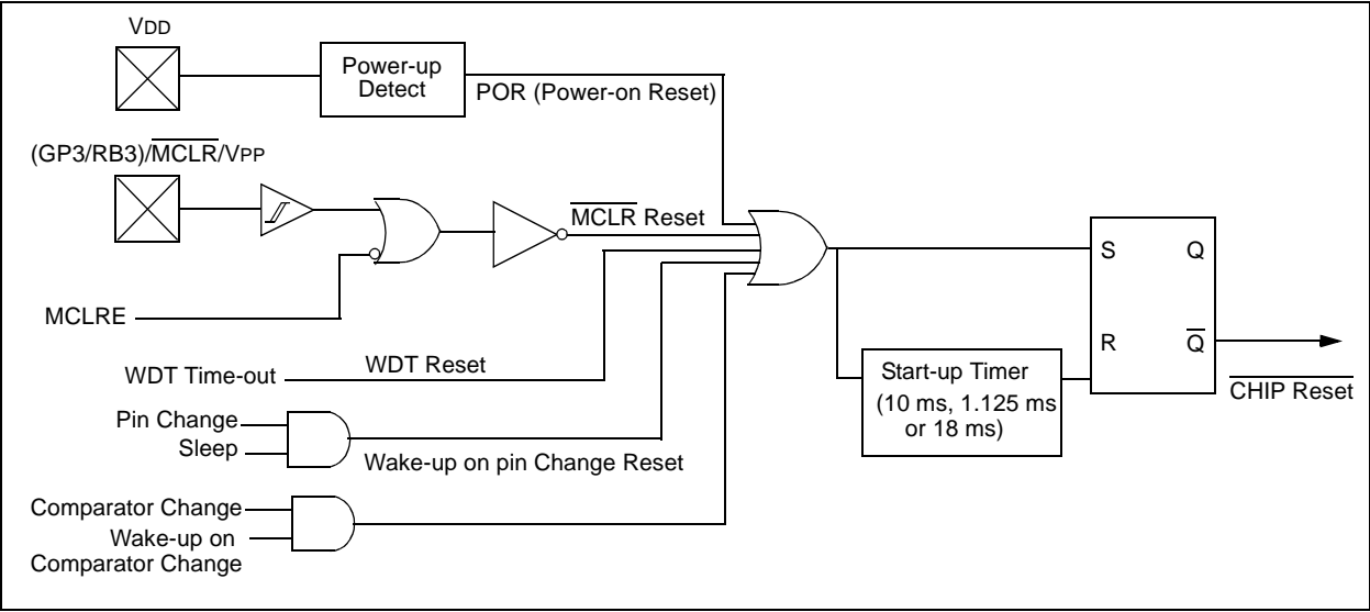
FIGURE 10-9: TIME-OUT SEQUENCE ON POWER-UP ( \overline{\text{MCLR}} PULLED LOW)
