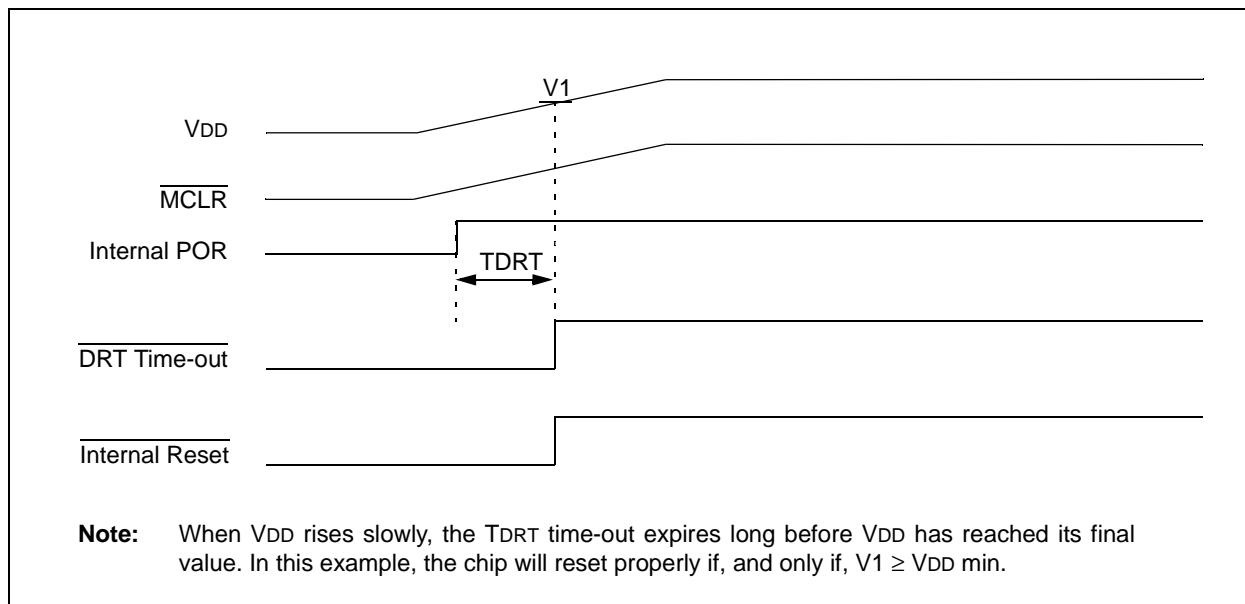
FIGURE 10-11: TIME-OUT SEQUENCE ON POWER-UP ( \overline{\text{MCLR}} TIED TO V_{\text{DD}} ): SLOW V_{\text{DD}} RISE TIME
