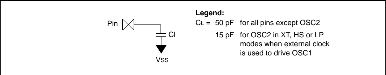
FIGURE 13-5: LOAD CONDITIONS
