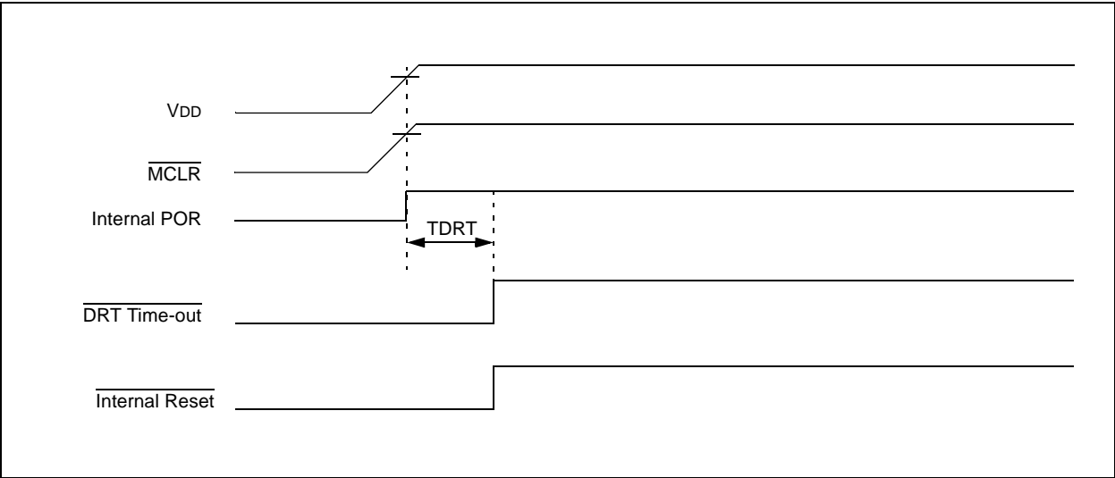
FIGURE 10-10: TIME-OUT SEQUENCE ON POWER-UP ( \overline{\text{MCLR}} TIED TO \text{VDD} ): FAST \text{VDD} RISE TIME
