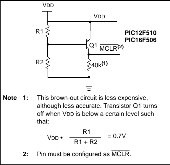
FIGURE 10-15: BROWN-OUT PROTECTION CIRCUIT 3
