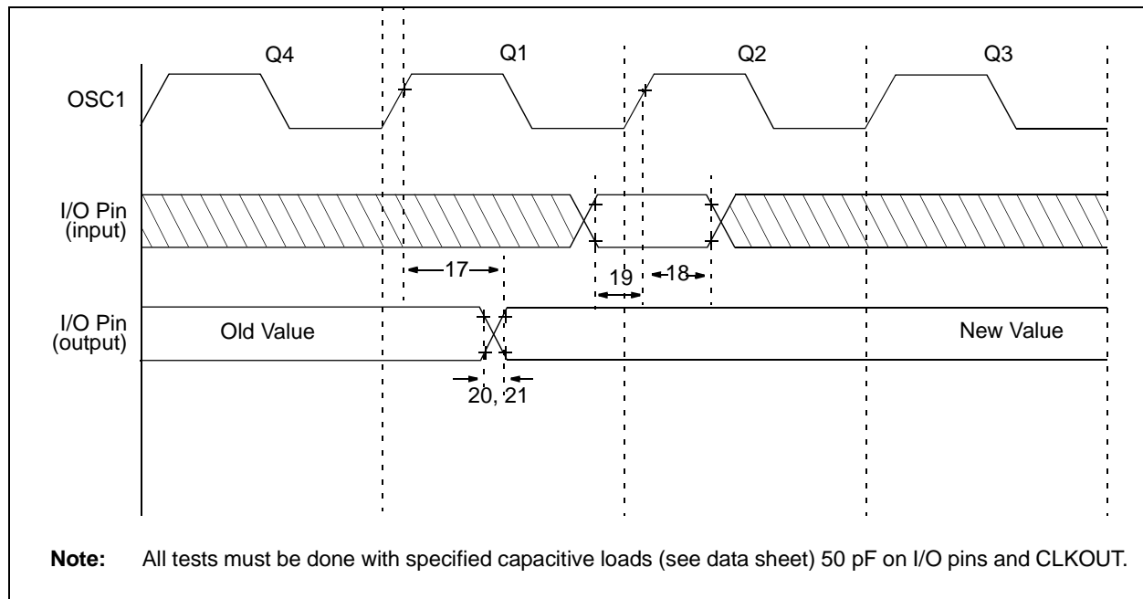
FIGURE 13-7: I/O TIMING
