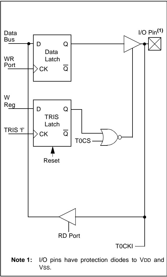
FIGURE 5-13: BLOCK DIAGRAM OF RC5
