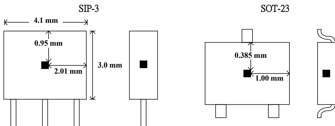
Fig. 1 SENSOR LOCATIONS
