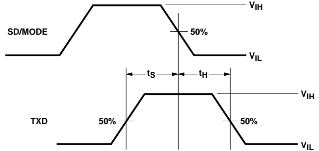
Figure 4. Bandwidth selection timing at FIR mode.
