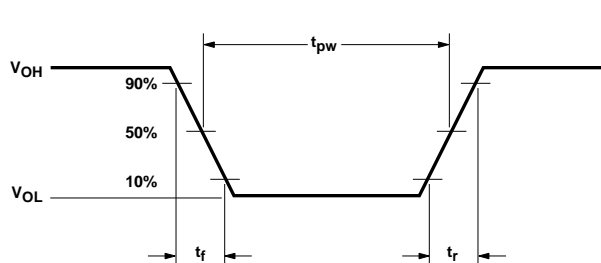
Figure 7. RXD output waveform.
