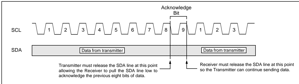
FIGURE 3-2: ACKNOWLEDGE TIMING
