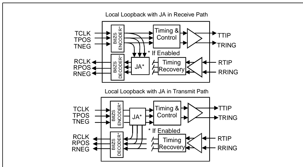
Figure 6. Local Loopback
