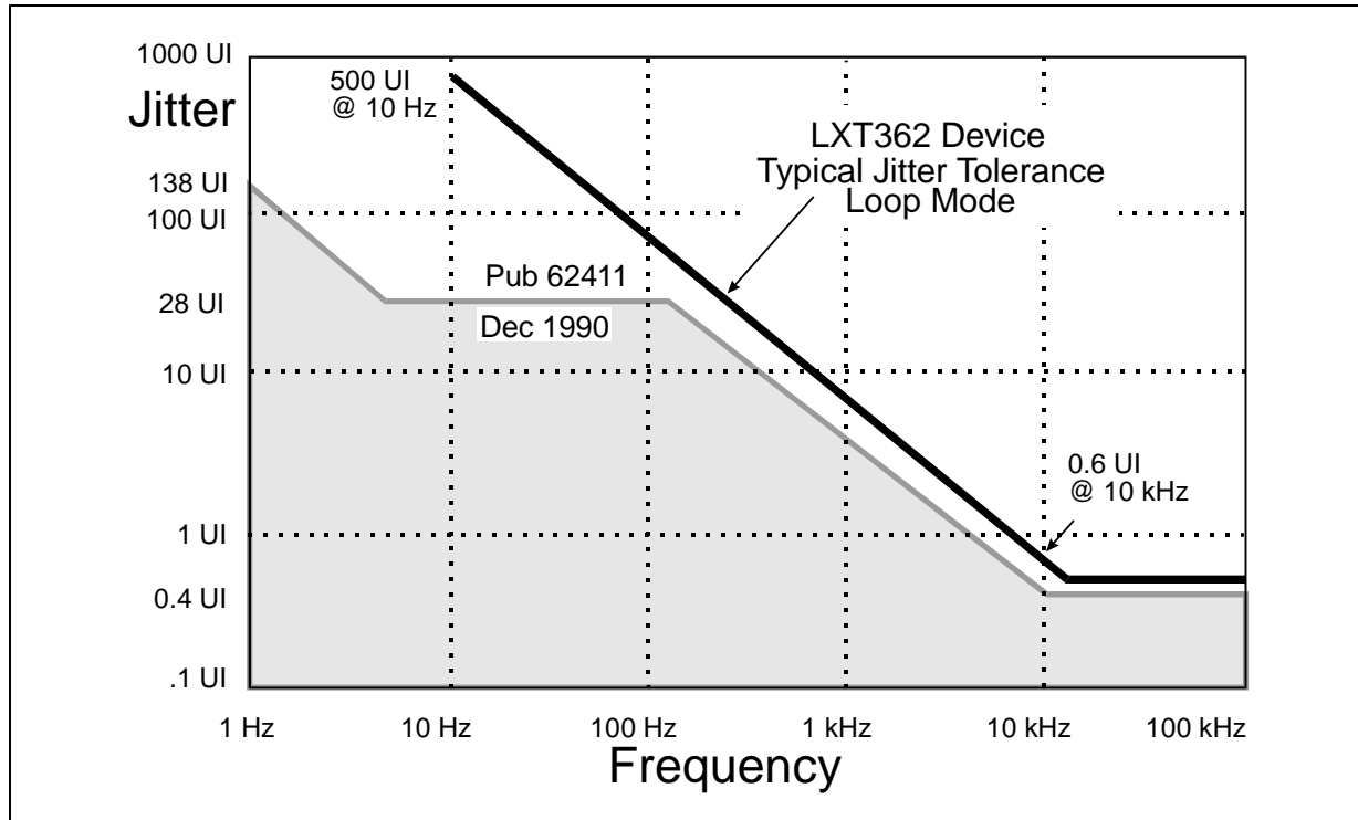
Figure 19. Typical T1 Jitter Tolerance at 36 dB
