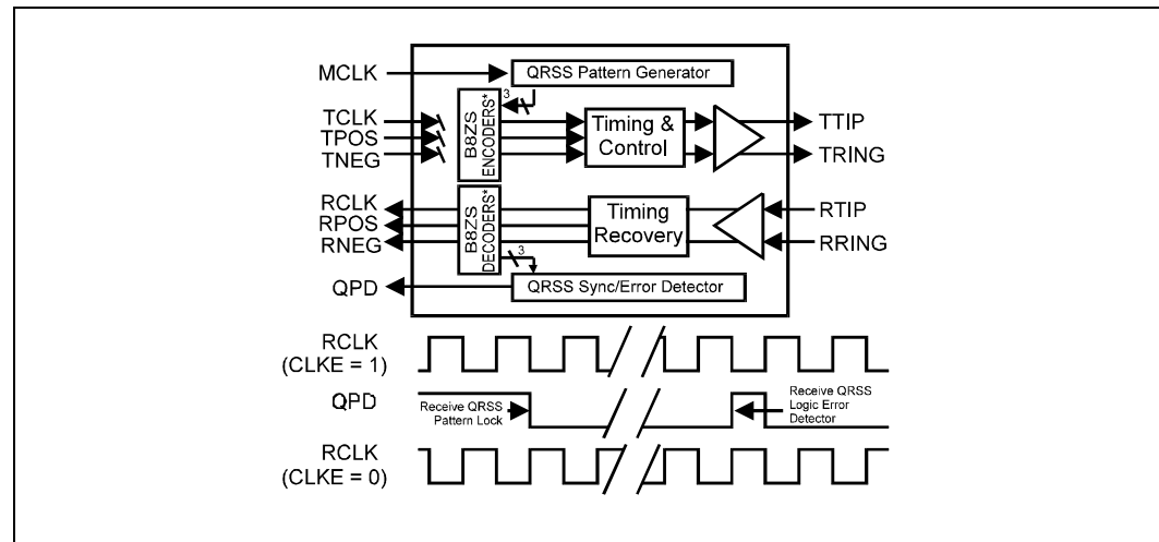
Figure 11. QRSS Mode
