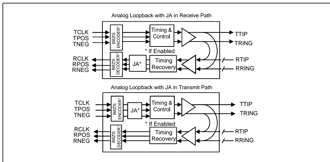
Figure 7. Analog Loopback
