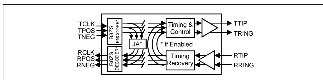
Figure 9. Dual Loopback
