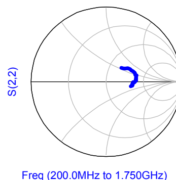
Figure 9. S22 vs. Output Frequency ( V_{DD} = 3\text{ V} )
