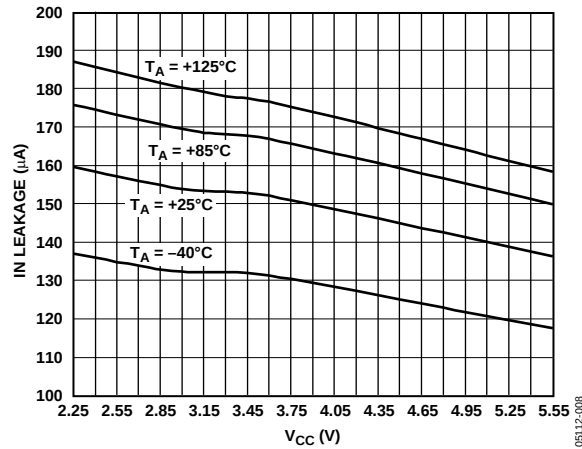
Figure 9. Input Leakage vs. Supply Voltage ( V_{IN} = 22 V )
