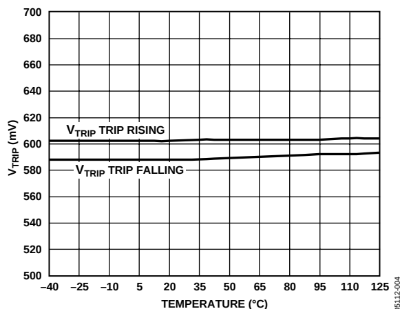
Figure 4. V_{IN} Trip Threshold vs. Temperature. ( V_{CC} = 3.3V )
