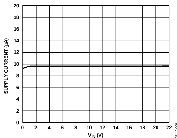
Figure 6. Supply Current vs. Input Voltage
