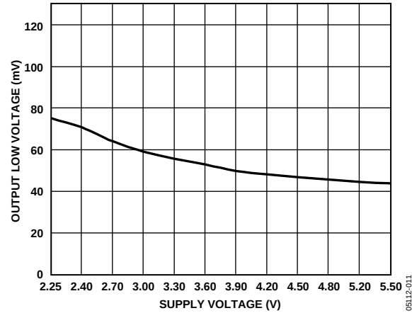
Figure 13. Output Low Voltage vs. Supply Voltage ( I_{SINK} = 500 mA )
