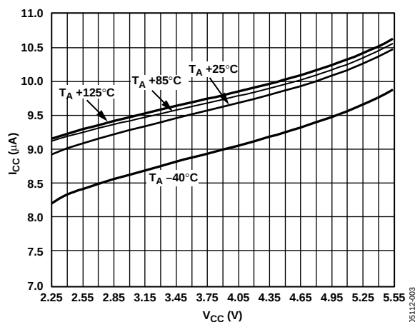
Figure 3. I_{CC} vs. V_{CC} over Temperature.
