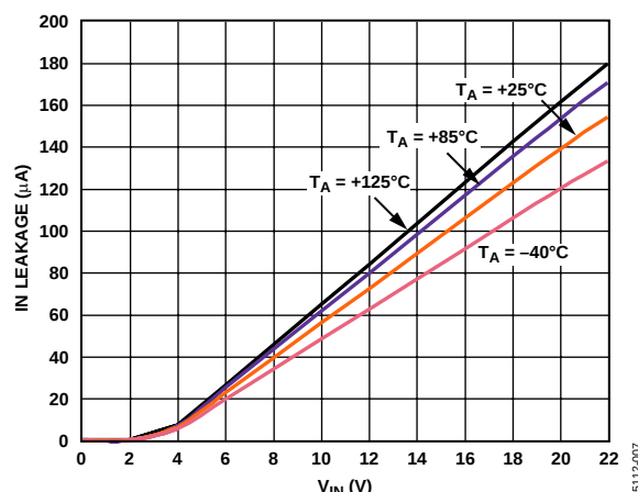
Figure 7. Input Leakage vs. Input Voltage
