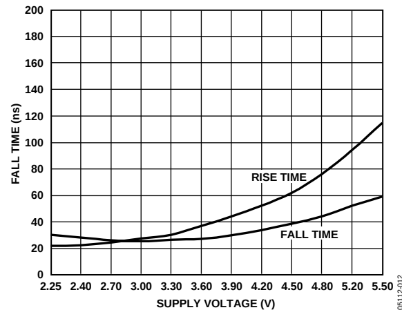
Figure 14. Fall Time vs. Supply Voltage
