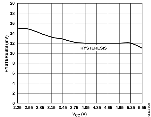
Figure 11. V_{IN} Trip Hysteresis vs. V_{CC}
