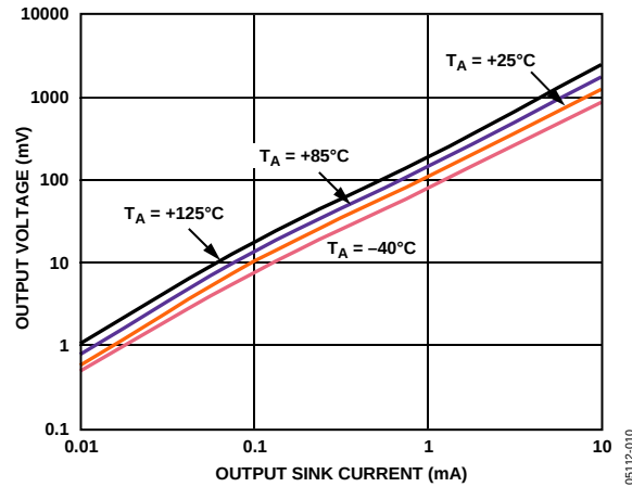
Figure 12. Output Voltage vs. Output Sink Current ( I_{SINK} = 500 mA )
