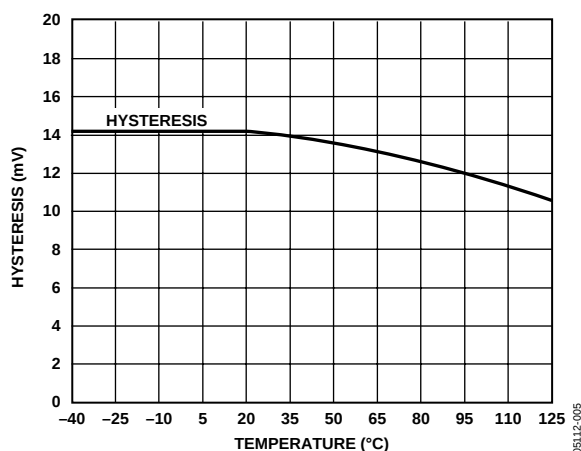
Figure 5. V_{IN} Trip Hysteresis vs. Temperature
