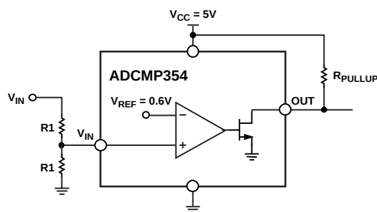
Figure 20. Voltage Detector Application
