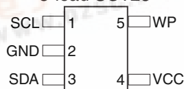
5-lead SOT23
