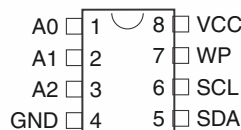
8-lead PDIP
