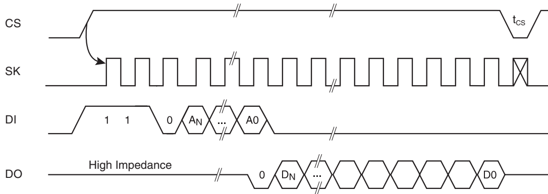
Figure 3. READ Timing
