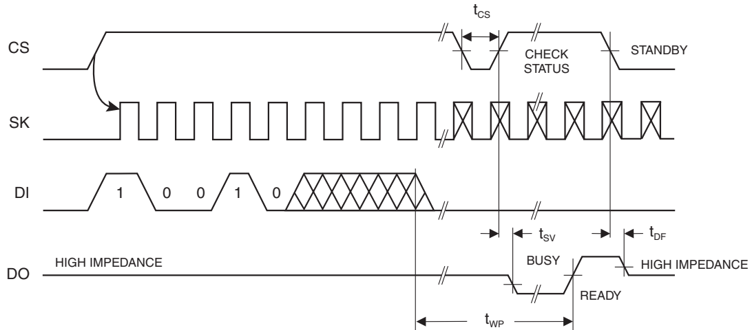
Figure 9. ERAL Timing (1)
