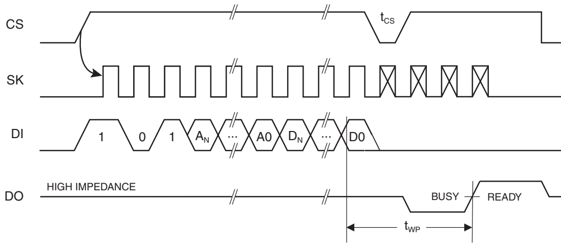
Figure 6. WRITE Timing
