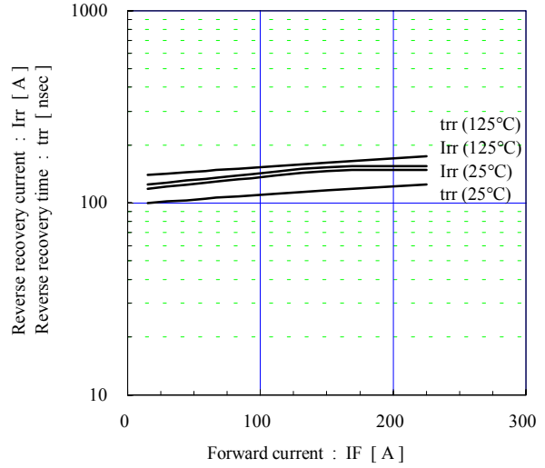
Reverse recovery characteristics (typ.) V_{ce}=600\text{V} , V_{GE}=\pm 15\text{V} , R_g=4.7\Omega
