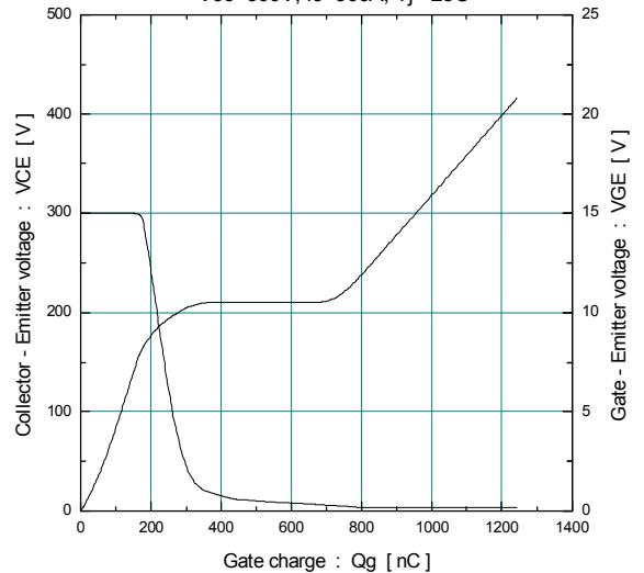
[ Inverter ] Dynamic Gate charge (typ.) Vcc=300V, Ic=300A, Tj= 25C
