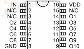
3D7110S SOL (300 Mil)
