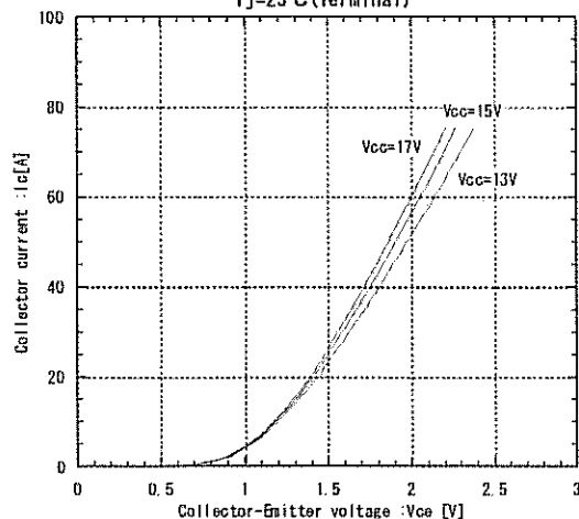
Collector current vs. Collector-Emitter voltage (typ.) T_J = 25^\circ\text{C} (Terminal)
