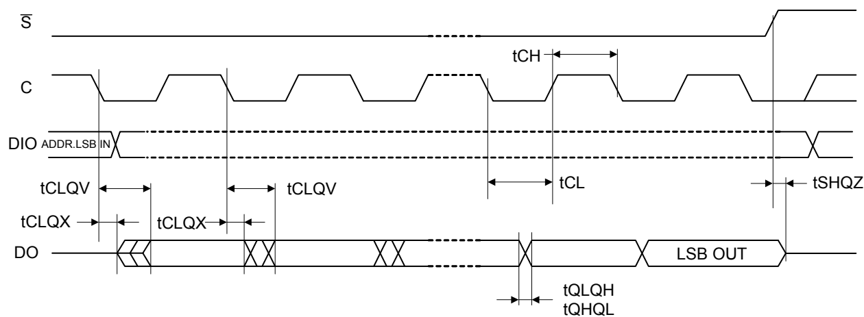
Figure 24. Output Timing
