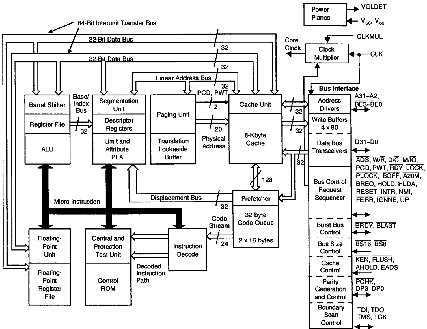
Am486 CPU Pipelined 32-Bit Microarchitecture
