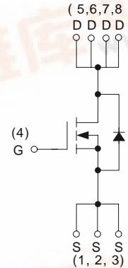
N-Channel MOSFET
