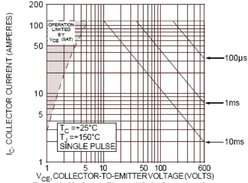
Figure 4, Maximum Forward Safe Operating Area
