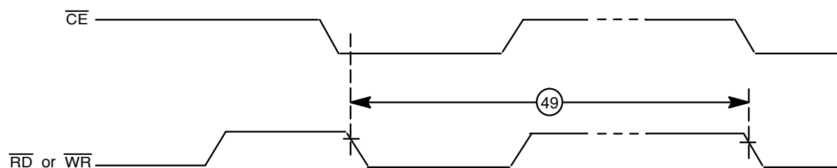
Figure 22. Reset Timing
