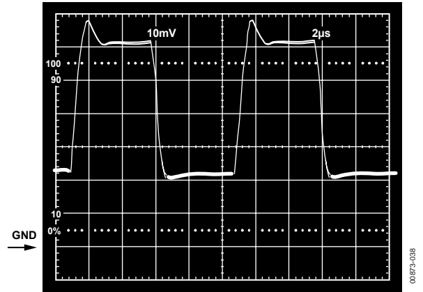
Figure 37. V_S = 5\text{ V}, 0\text{ V} ; Gain of Two Inverter Response to 20 mV Step, Centered 20 mV Below Ground
