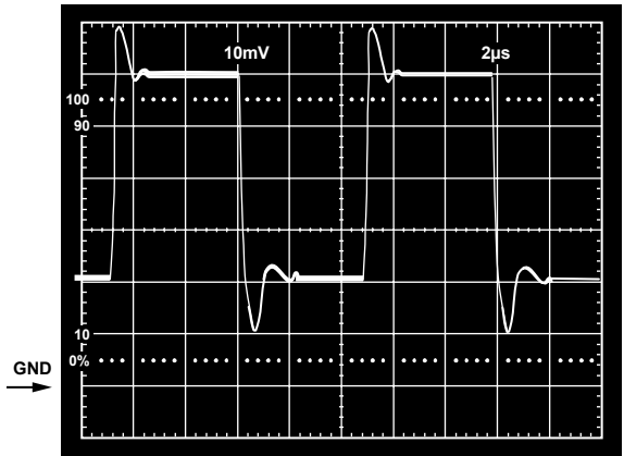
Figure 34. V_S = 5\text{ V}, 0\text{ V} ; Unity-Gain Follower Response to 40 mV Step Centered 40 mV Above Ground
