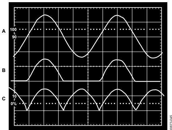
Figure 44. Single-Supply Half- and Full-Wave Rectifier
