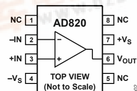
Figure 2. 8-Lead SOIC
