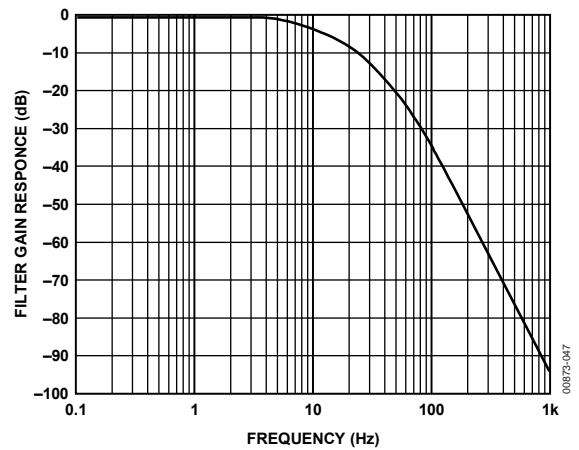
Figure 46. 10 Hz Sallen Key Low-Pass Filter
