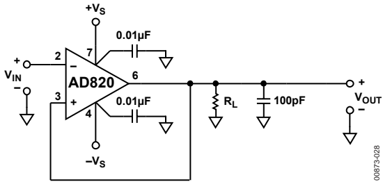
Figure 27. Unity-Gain Follower, Used for Figure 28 Through Figure 32
