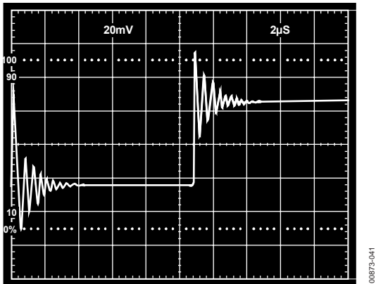
Figure 40. Small Signal Response of AD820 as Unity-Gain Follower Driving 350 pF Capacitive Load
