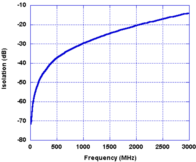
Figure 10. Isolation – Input to Output
