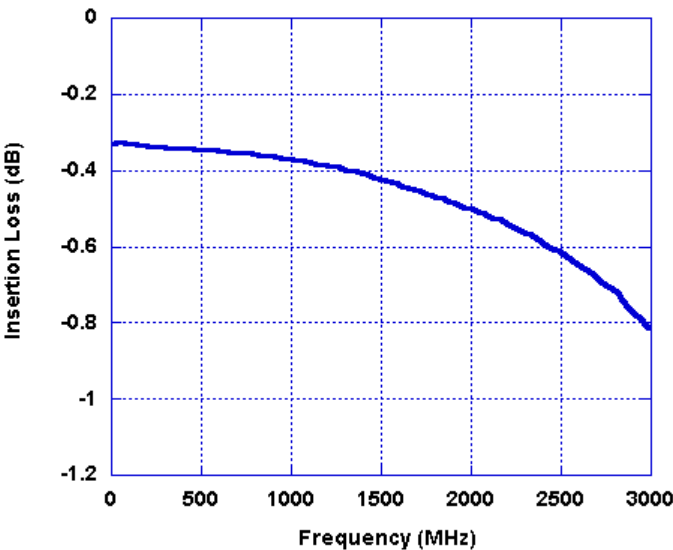
Figure 9. Insertion Loss
