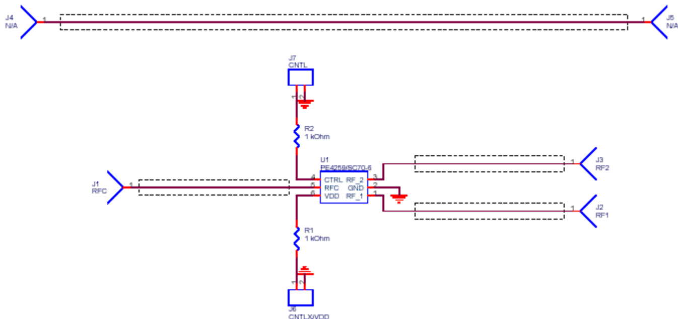
Figure 9. Evaluation Board Schematic
