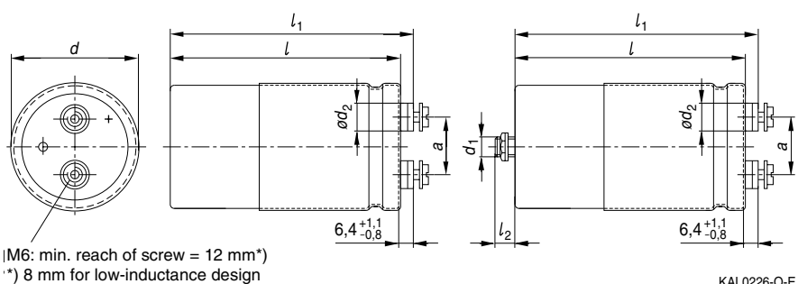
Type B43750 Ring clip/clamp mounting
