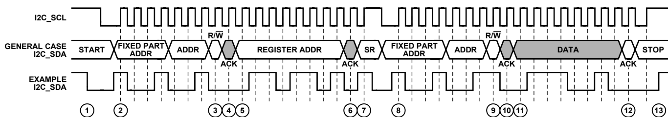
Figure 30. I²C Read Diagram
