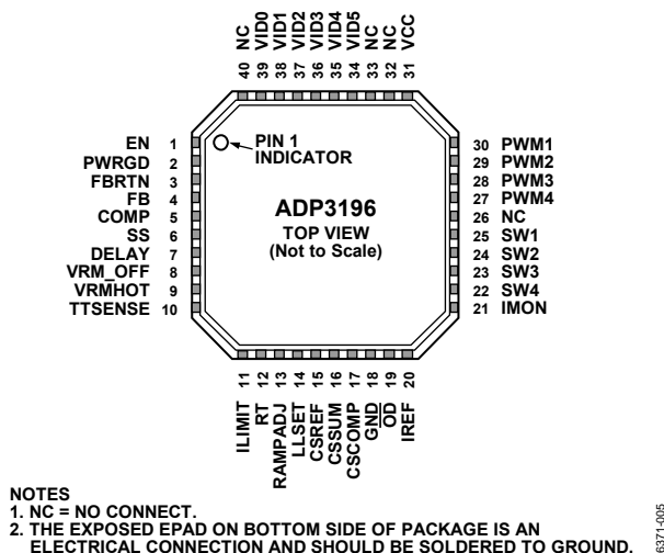
Figure 5. Pin Configuration
