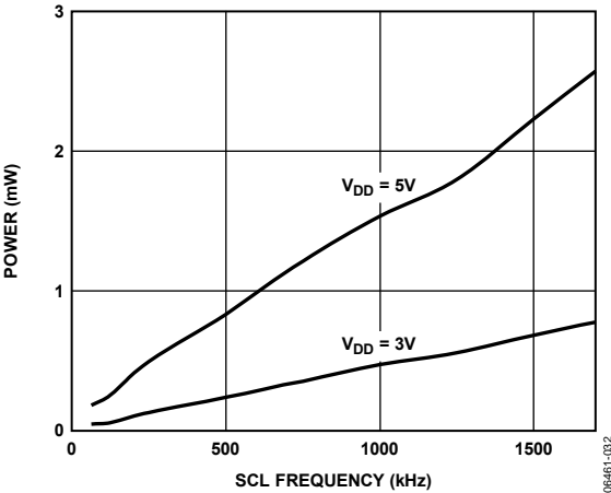
Figure 17. Power vs. SCL Frequency, V_{REF} = 2.5\text{ V}
