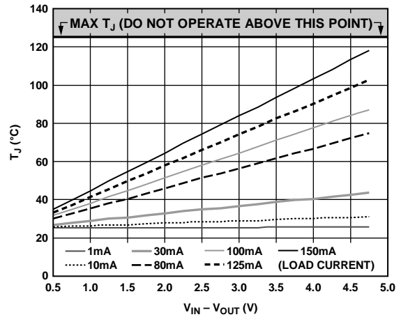
Figure 23. 500 mm 2 of PCB Copper, T_A = 25^\circ\text{C}
