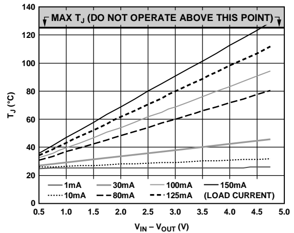
Figure 24. 100 mm 2 of PCB Copper, T_A = 25^\circ\text{C}
