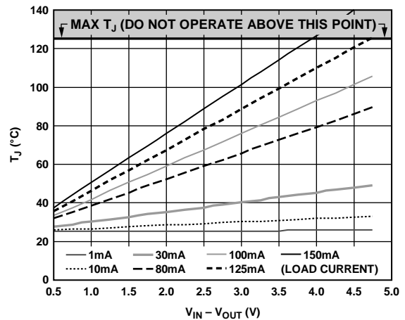
Figure 25. 0 mm 2 of PCB Copper, T_A = 25^\circ\text{C}
