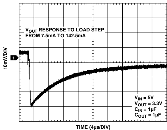
Figure 21. Output Transient Response, C_{\text{OUT}} = 1 \mu\text{F}
