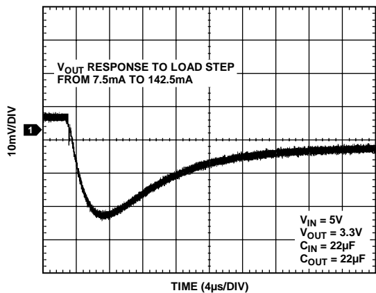
Figure 22. Output Transient Response, C_{\text{OUT}} = 22 \mu\text{F}
