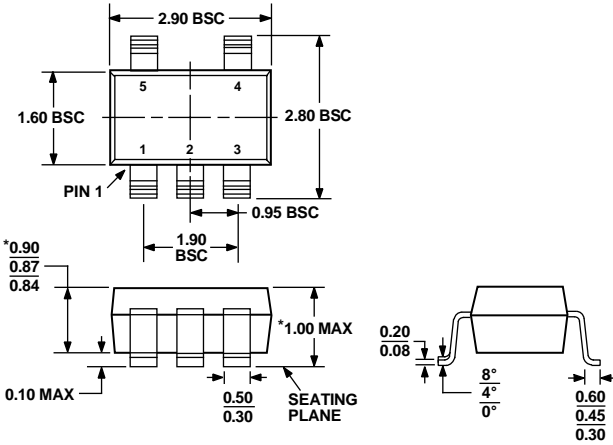
Figure 30. 5-Lead Thin Small Outline Transistor Package [TSOT] (UJ-5) Dimensions show in millimeters
