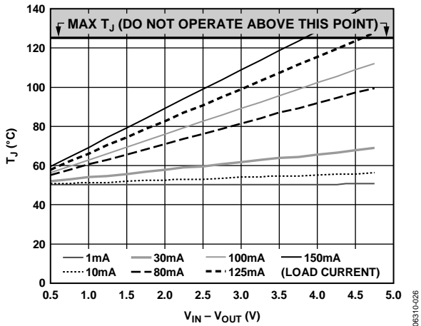
Figure 26. 500 mm 2 of PCB Copper, T A = 50°C
