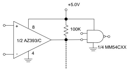
Figure 10. Driving CMOS/TTL
