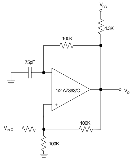
Figure 12. Squarewave Oscillator
