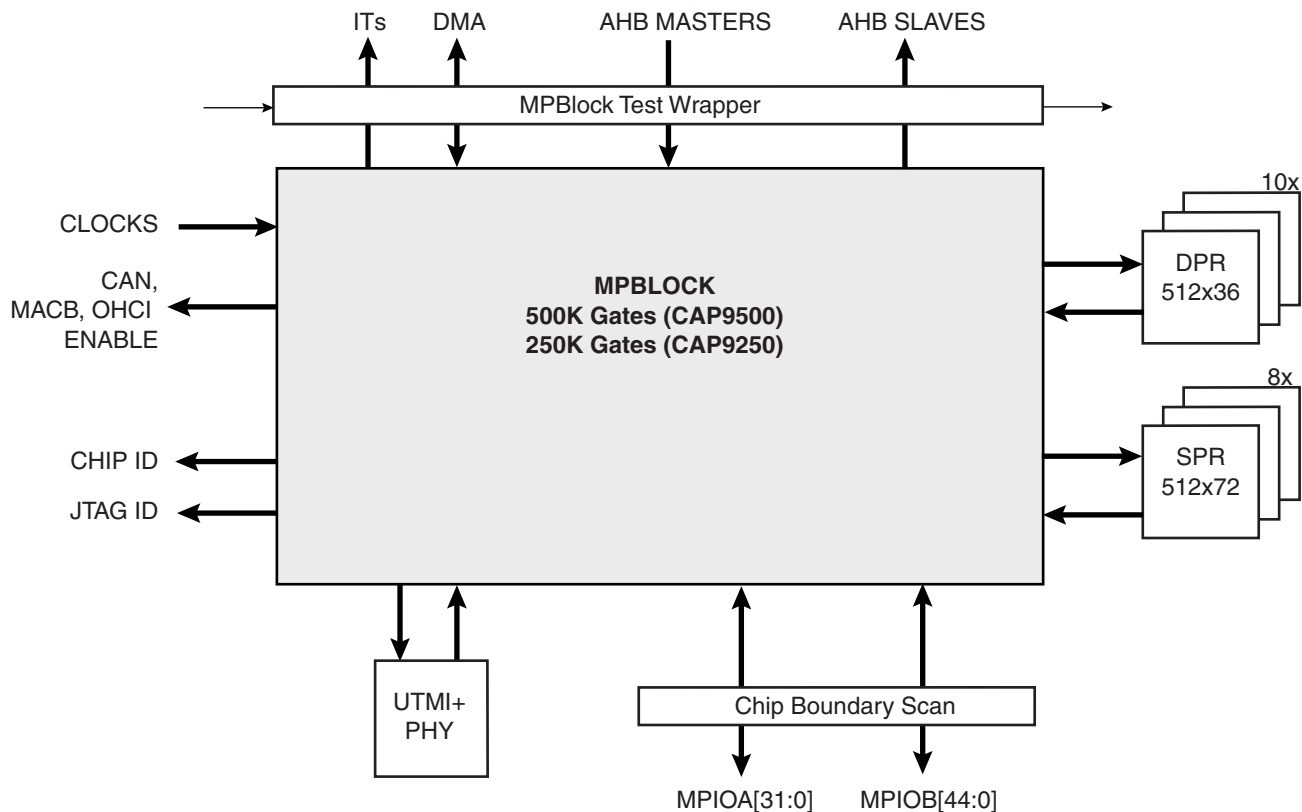
Figure 11-1. MPBlock Connectivity
