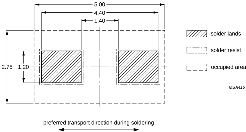
Fig 16. Wave soldering footprint SOD323 (SC-76)
