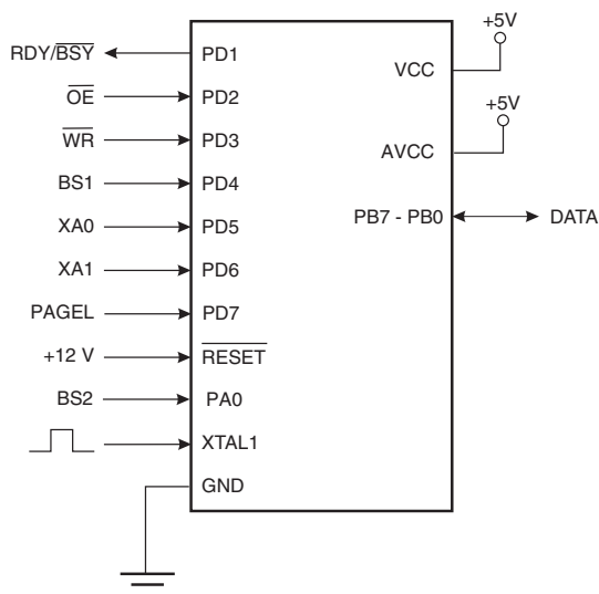
Figure 26-1. Parallel Programming
