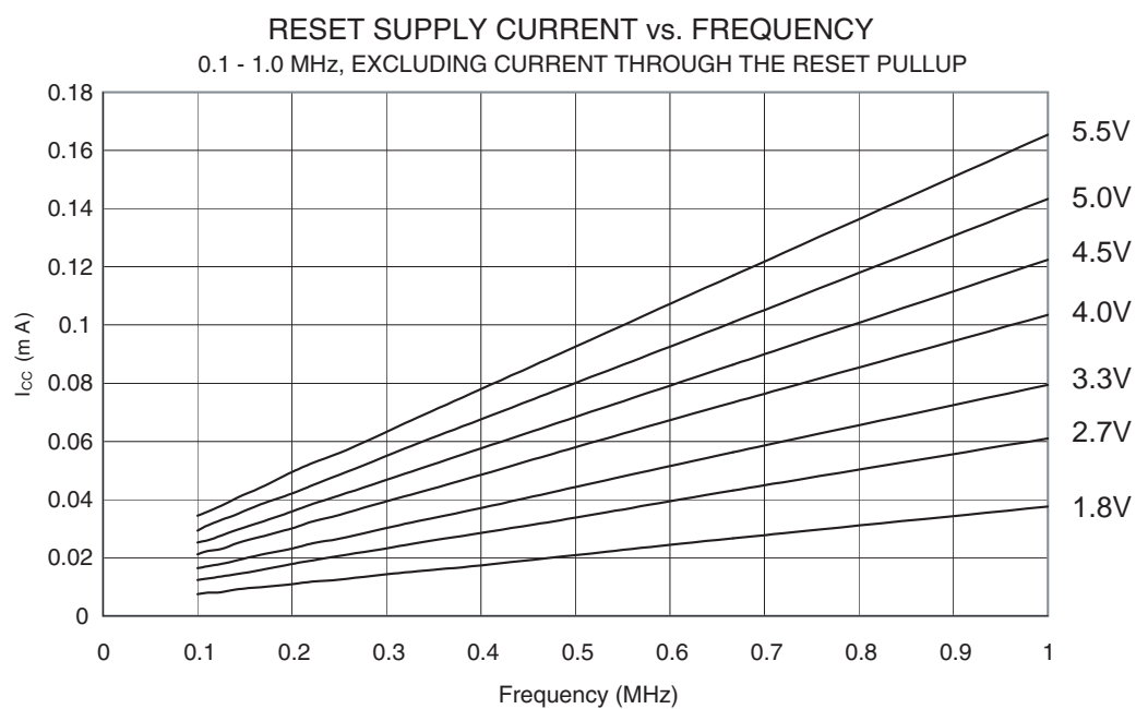
Figure 28-65. Reset Supply Current vs. V_{CC} (0.1 - 1.0 MHz, Excluding Current Through The Reset Pull-up)
