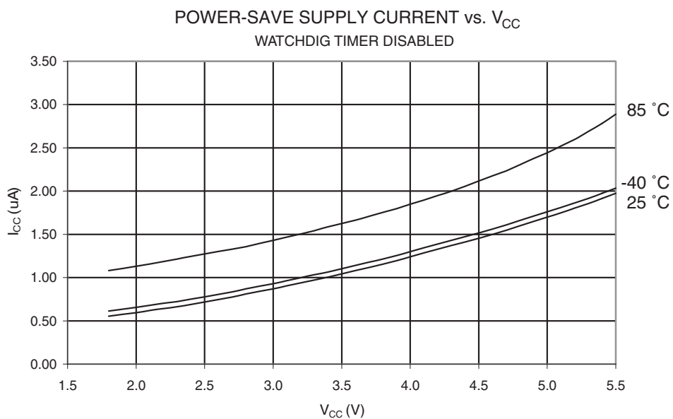
Figure 28-13. Power-save Supply Current vs. V_{CC} (Watchdog Timer Disabled)
