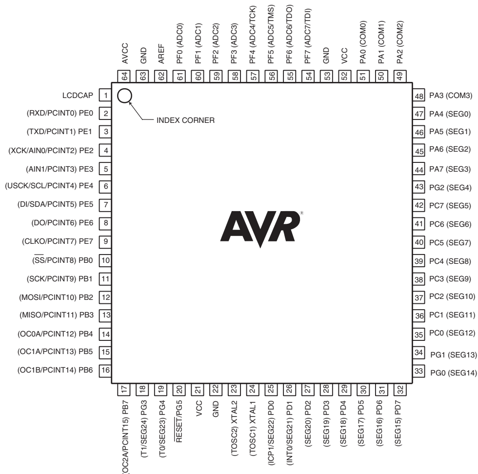
Figure 1-1. Pinout ATmega169P
