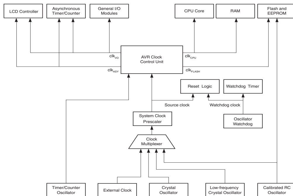
Figure 7-1. Clock Distribution
