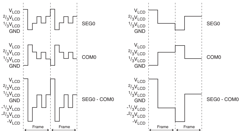
Figure 22-7. Default and Low Power Waveform
