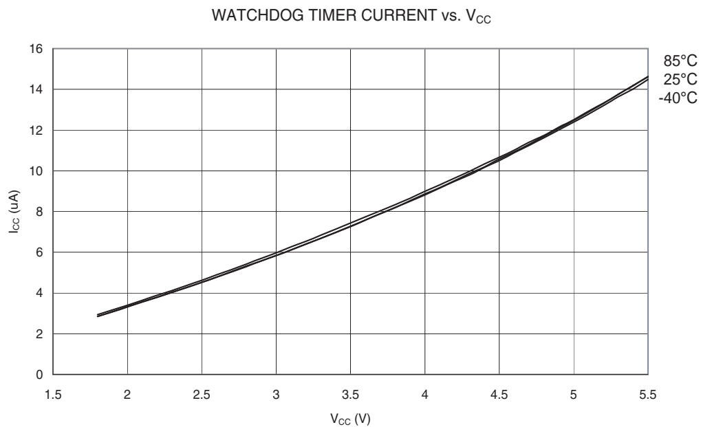
Figure 28-62. Watchdog Timer Current vs. V_{CC}
