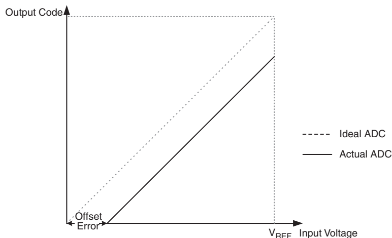
Figure 21-10. Offset Error
