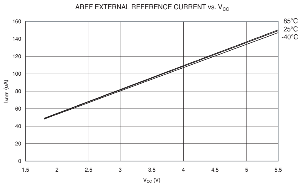
Figure 28-60. AREF External Reference Current vs. V_{CC}
