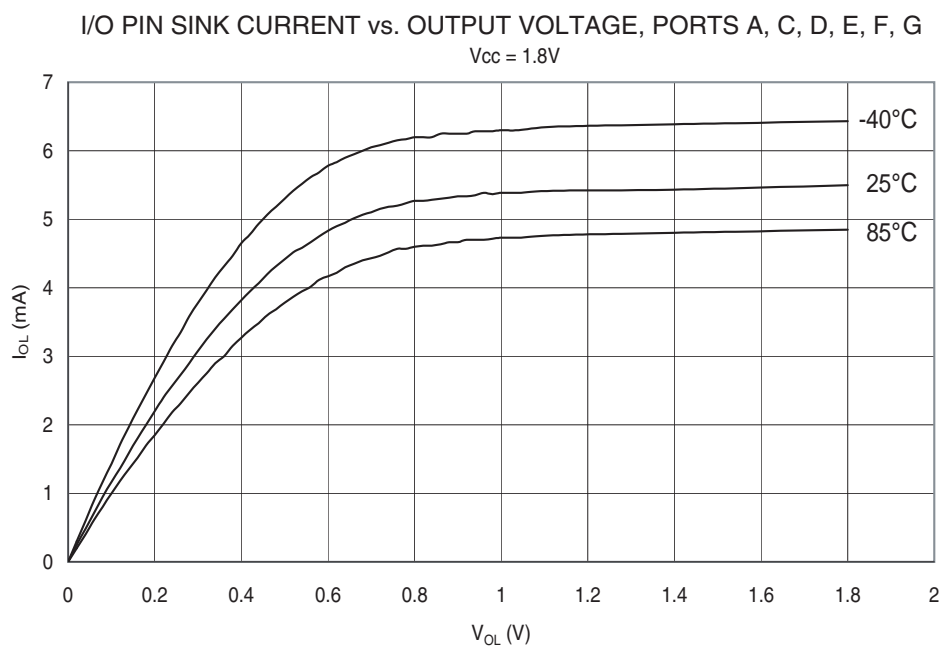
Figure 28-37. I/O Pin Sink Current vs. Output Voltage, Ports A, C, D, E, F, G ( V_{CC} = 1.8V )
