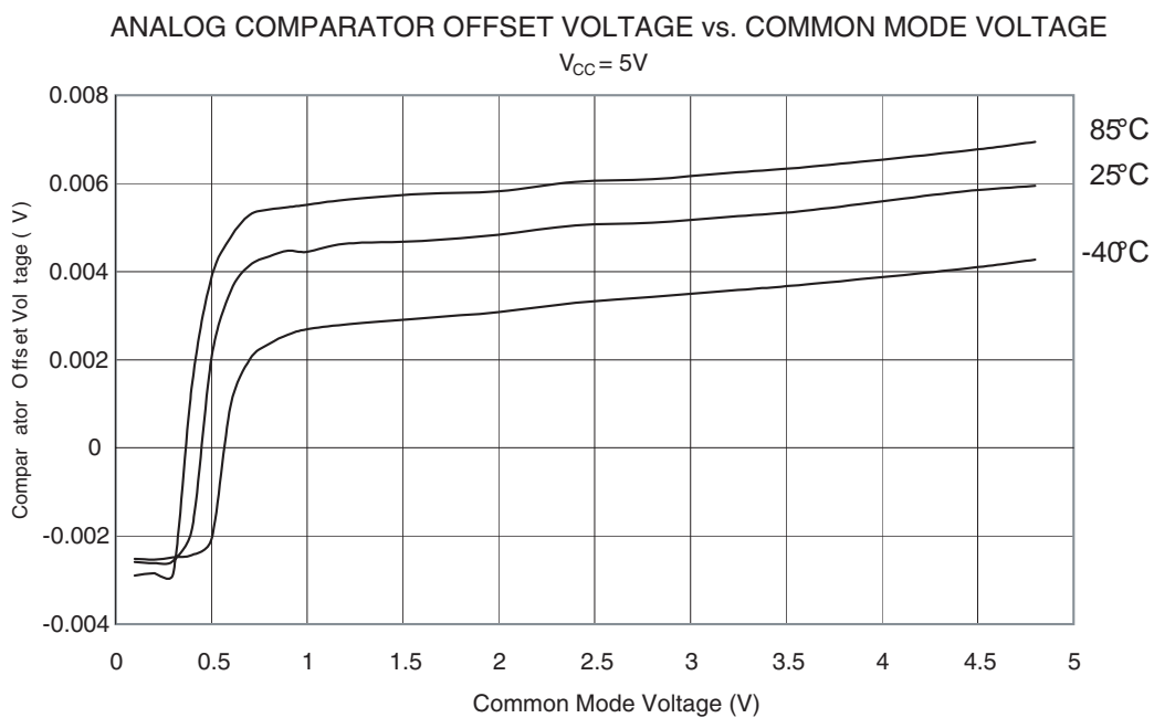
Figure 28-51. Analog Comparator Offset Voltage vs. Common Mode Voltage ( V_{CC} = 5V )
