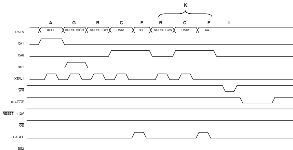
Figure 26-4. Programming the EEPROM Waveforms
