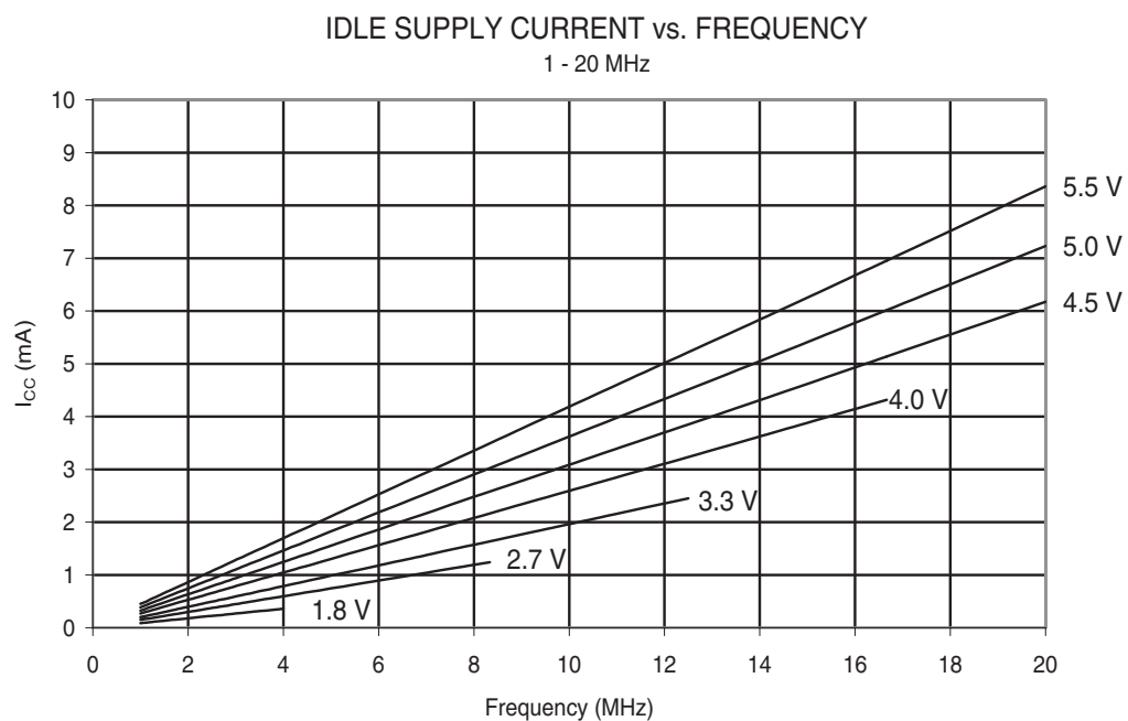
Figure 28-7. Idle Supply Current vs. Frequency (1 - 20 MHz)
