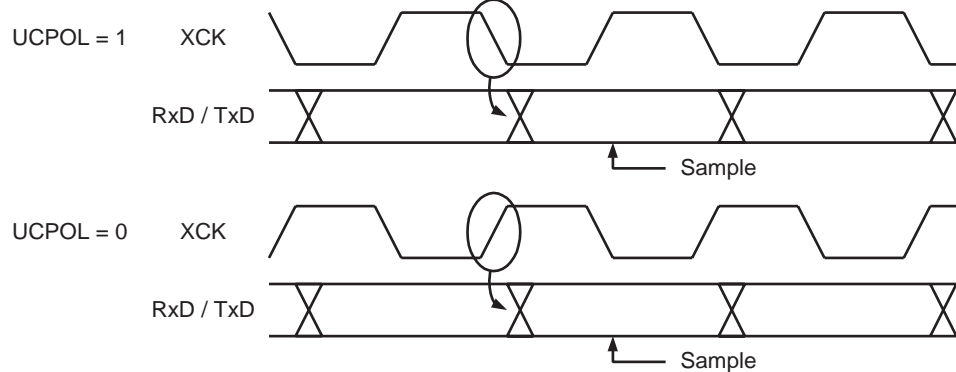
Figure 18-3. Synchronous Mode XCK Timing.
