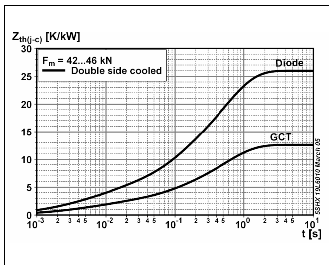
Fig. 1 Transient thermal impedance (junction-to-case) vs. time (max. values) Note 1
