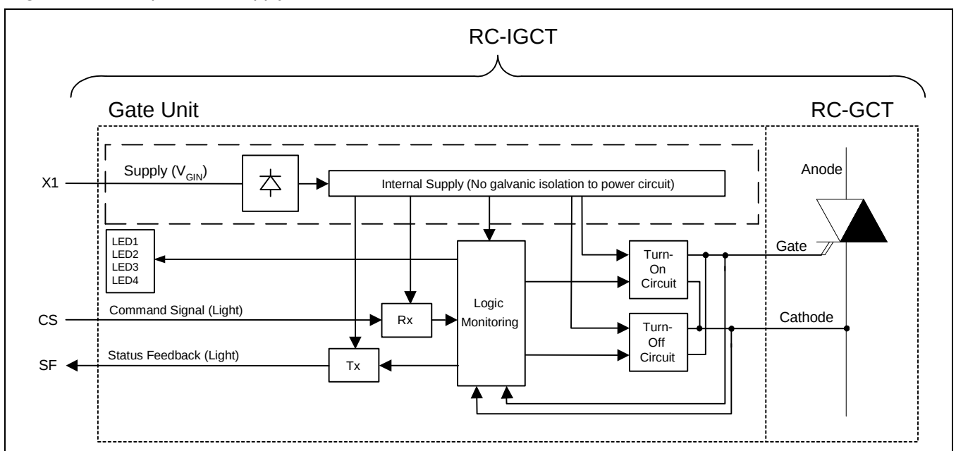
Fig. 22 Block diagram
