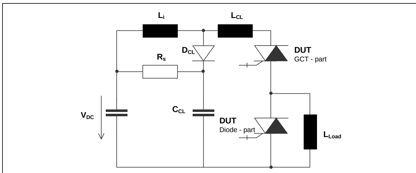
Fig. 25 Test circuit
