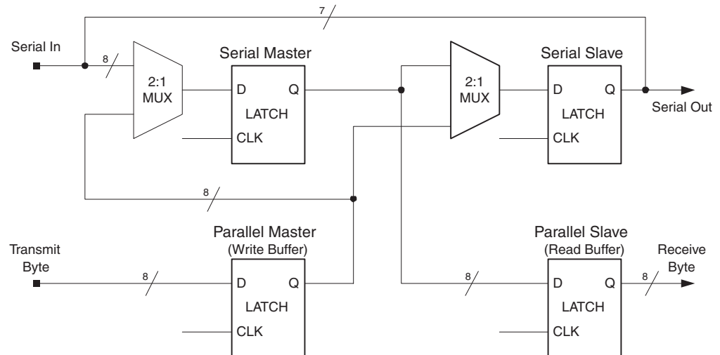
Figure 18-2. SPI Shift Register Diagram
