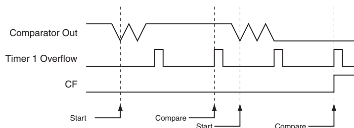
Figure 19-1. Negative Edge with Debouncing Example
