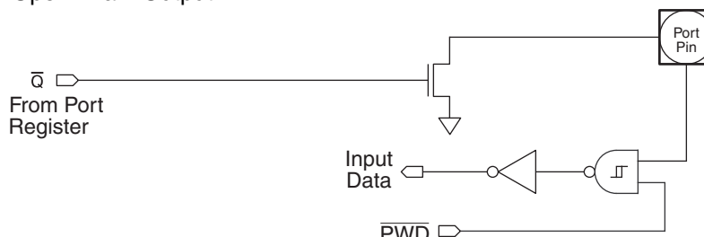
Figure 13-4. Open-Drain Output
