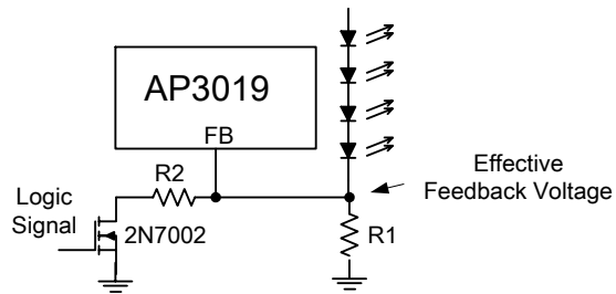
Figure 26. Dimming Control Using Logic Signal
