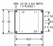
Dimensions, mm
