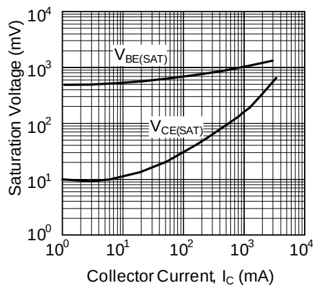
Saturation Voltage
