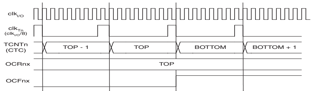
Figure 16-11. Timer/Counter Timing Diagram, Clear Timer on Compare Match mode, with Prescaler ( f_{clk\_I/O}/8 )
