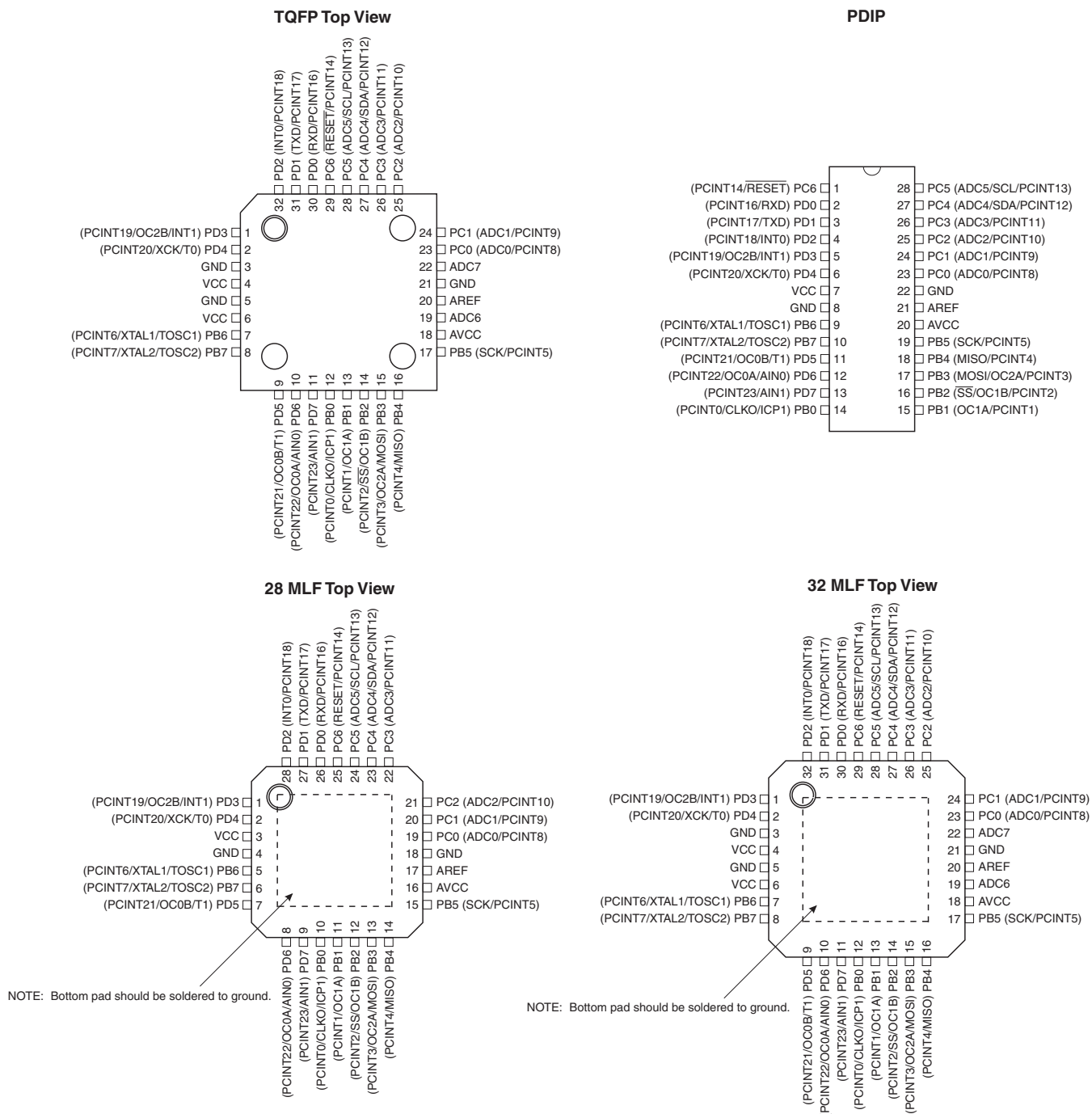
Figure 1-1. Pinout ATmega48/88/168
