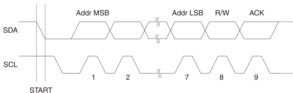
Figure 20-4. Address Packet Format
