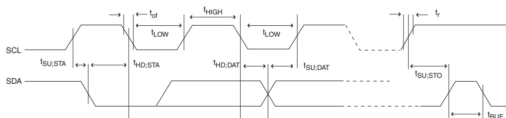
Figure 27-4. 2-wire Serial Bus Timing
