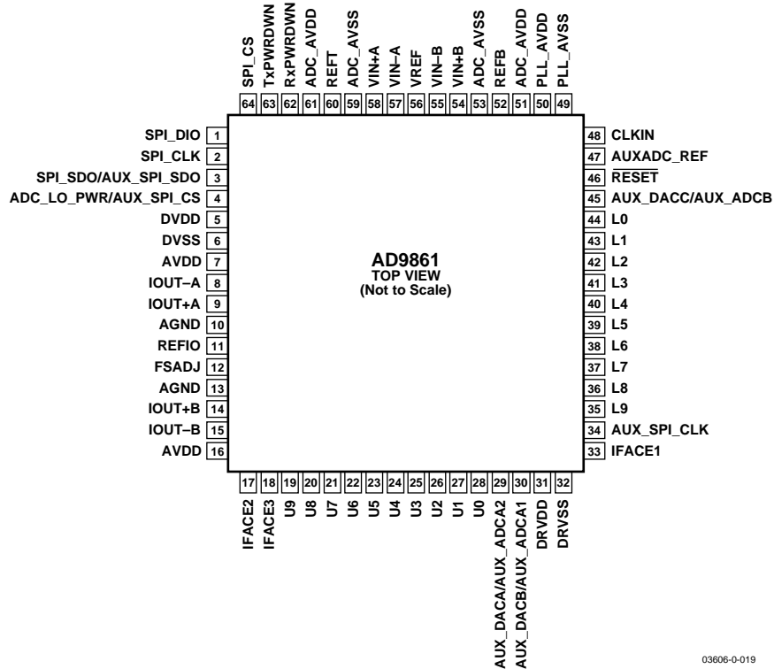
Figure 3. Pin Configuration
