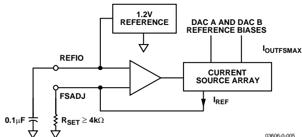
Figure 74. Reference Circuitry
