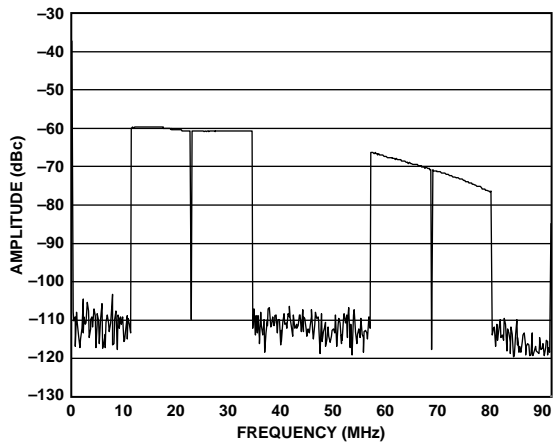
Figure 66. AD9861 Tx Path FFT of OFDM Signal in Figure 52 with 1 \times Interpolation
