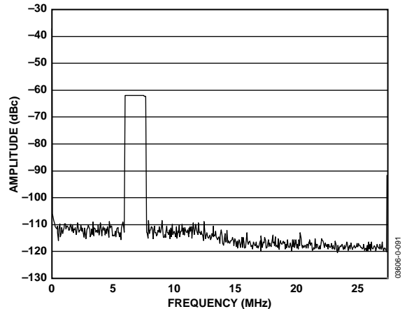
Figure 63. AD9861 Tx Path FFT of OFDM Signal in Figure 52, with 4 \times Interpolation
