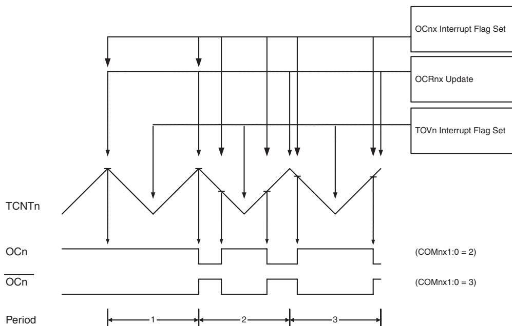
Figure 13-9. Phase Correct PWM Mode, Timing Diagram
