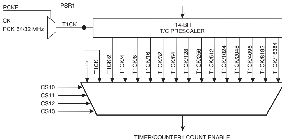
Figure 14-1. Timer/Counter1 Prescaler
