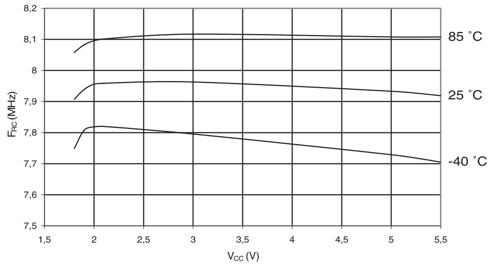
Figure 24-35. Calibrated 8 MHz RC Oscillator Frequency vs. Temperature
