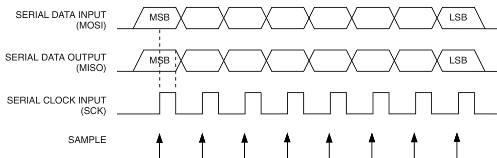
Figure 23-4. Serial Programming Waveforms
