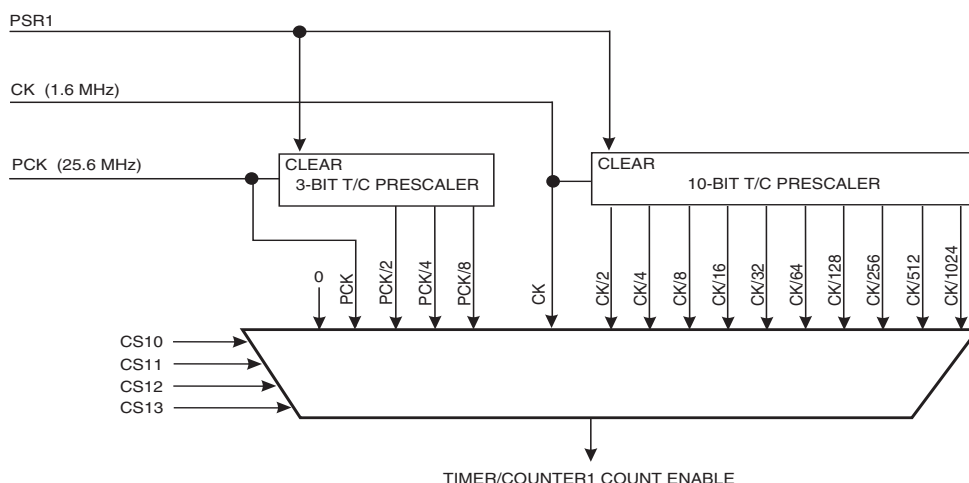
Figure 15-1. Timer/Counter1 Prescaler
