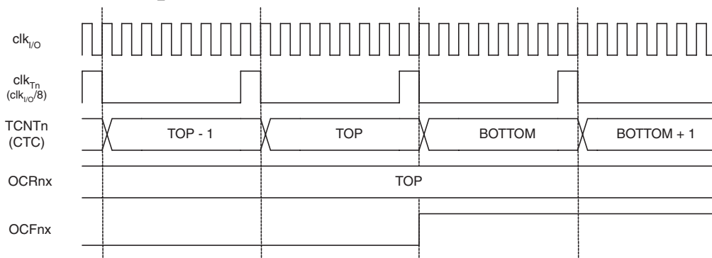
Figure 13-13. Timer/Counter Timing Diagram, Clear Timer on Compare mode, with Prescaler ( f_{clk\_I/O}/8 )
