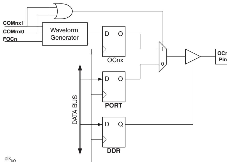
Figure 13-6. Compare Match Output Unit, Schematic
