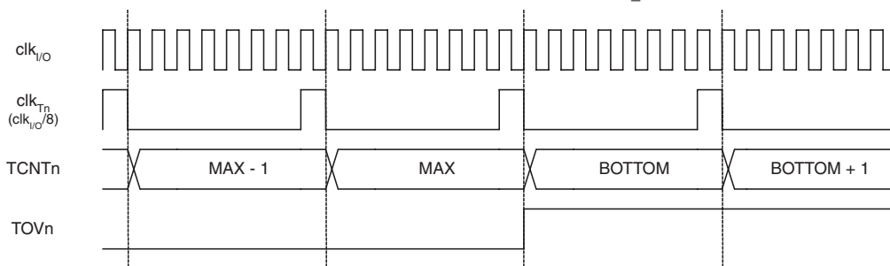
Figure 13-11. Timer/Counter Timing Diagram, with Prescaler ( f_{clk\_I/O}/8 )
