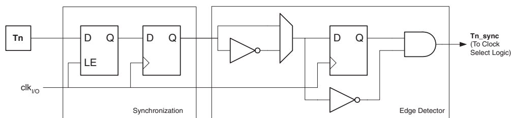
Figure 13-2. T0 Pin Sampling
