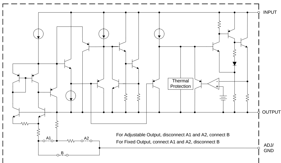
Figure 3. Functional Block Diagram of AZ1085
