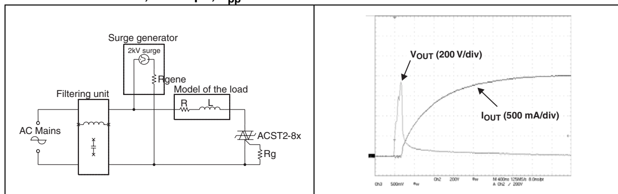
Figure 17. Typical current and voltage waveforms across the ACST2 during IEC 61000-4-5 standard test
