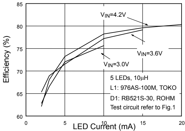
Fig. 10 5 LEDs Efficiency vs. LED Current
