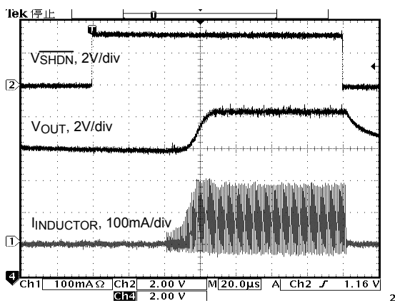
Fig. 12 Start-Up from Shutdown VIN=3.6V; 3 LEDs; L1=10µF; COUT=0.22µF; ILED=20mA
