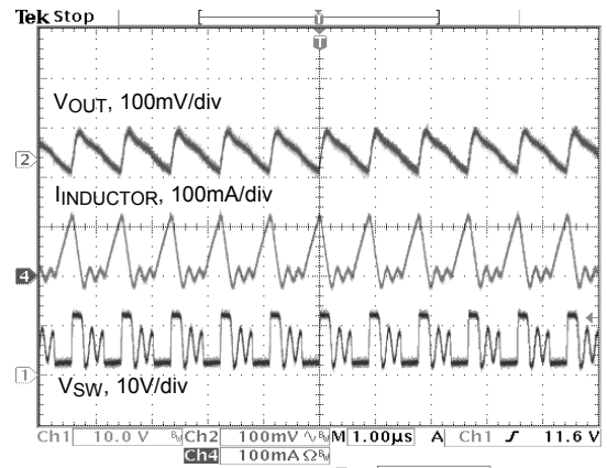
Fig. 13 Operation Wave Form VIN=3.6V; 3 LEDs; L1=10µF; COUT=0.22µF; ILED=10mA
